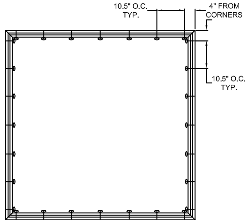
TYPICAL ELEVATION WITH FASTENER SPACING
